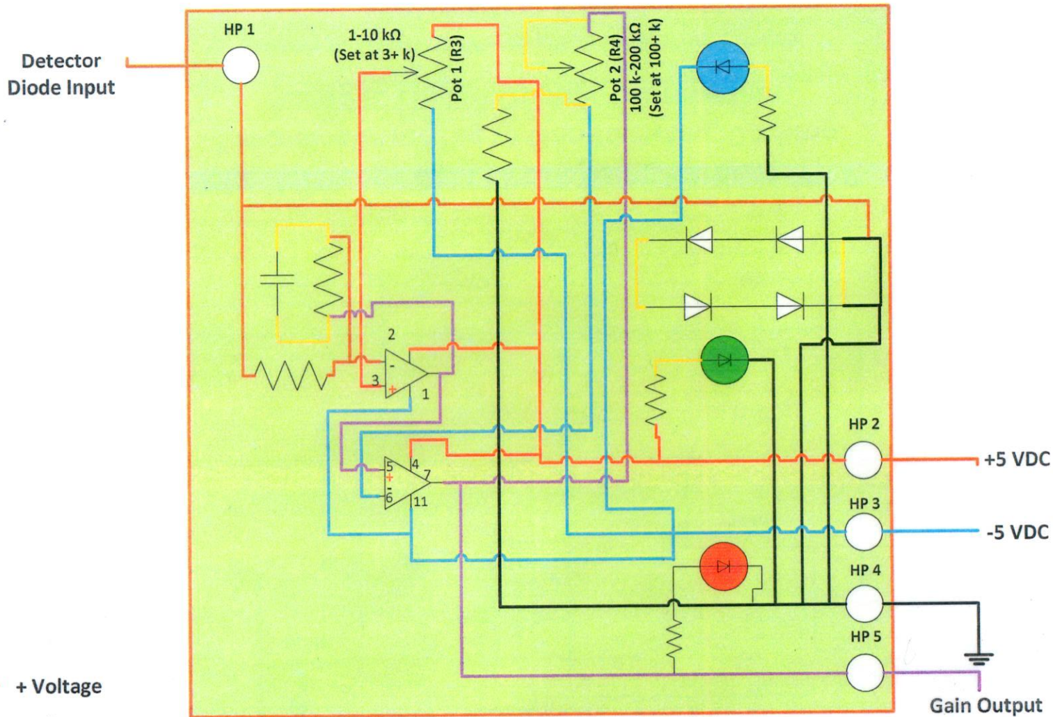
Solar Telescope Gain Circuit Using Hardwire PS & Cascading Inverting to Non-Inverting Op Amp (Quad IC LM324 Op Amp) Connection
